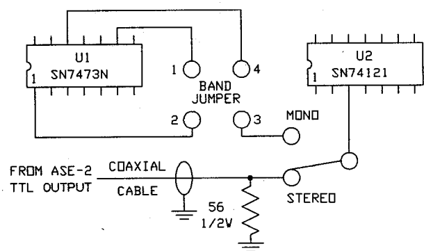
Figure 4-1 TTL Interface
